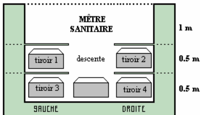
CAVEAU A CASES DOUBLES PLUS DESCENTE
